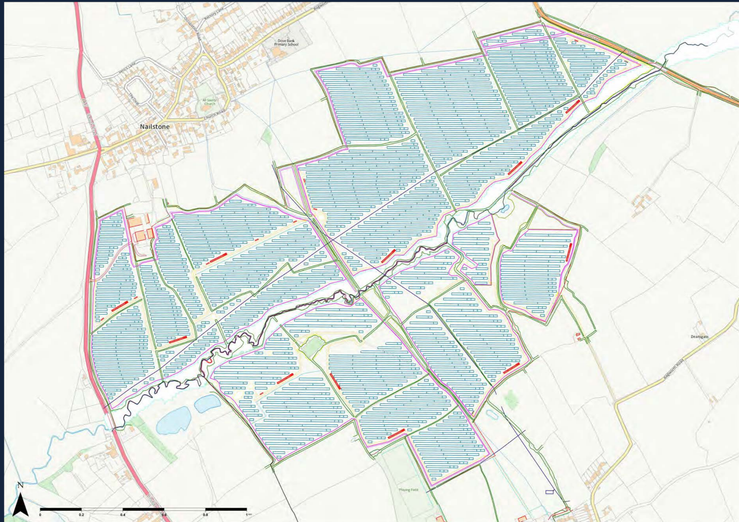
PV Layout Plan
